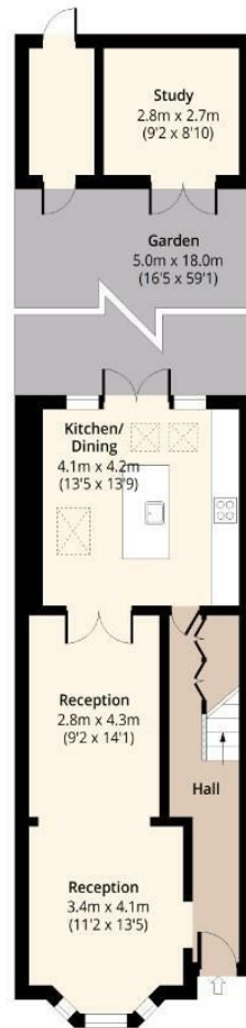
Ground Floor Approx. 54.44 Sq. meters (586 Sq. feet)
